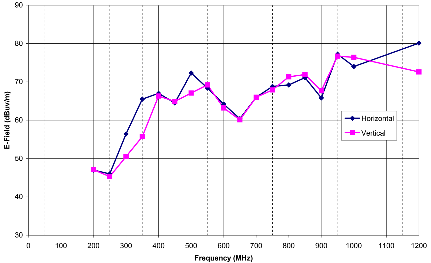
Typical PSDS E-Field at 10 meter Distance (Semianechoic Chamber) Receive Antenna Scanned from 1m to 4m
