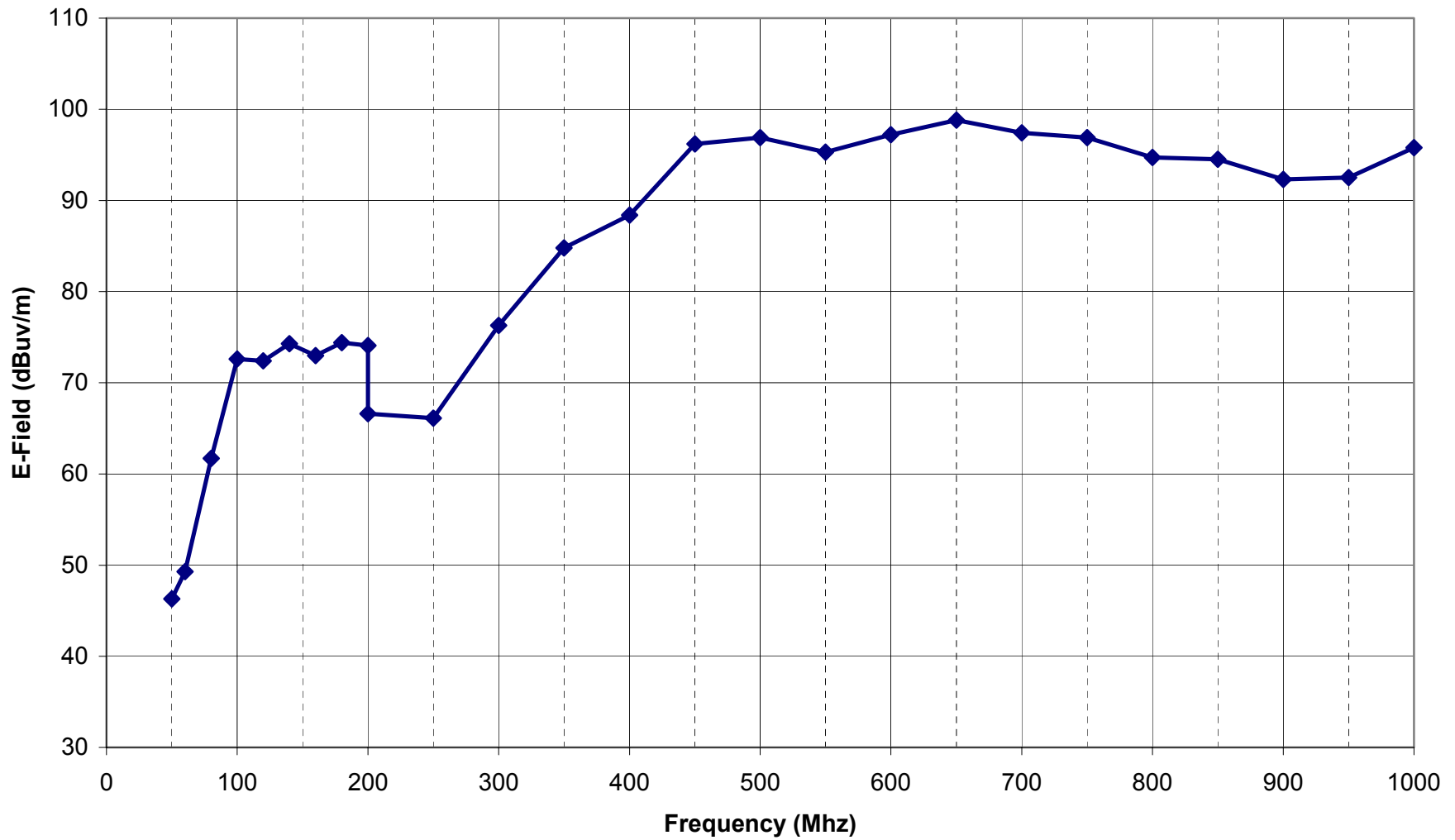
Typical PSDS Radiated E-Field at 1.5 m Horizontal Polarization (RF Generator = +10 dBm) Receive Antenna 1m Above Ground -- Sphere 0.8m Above Ground
