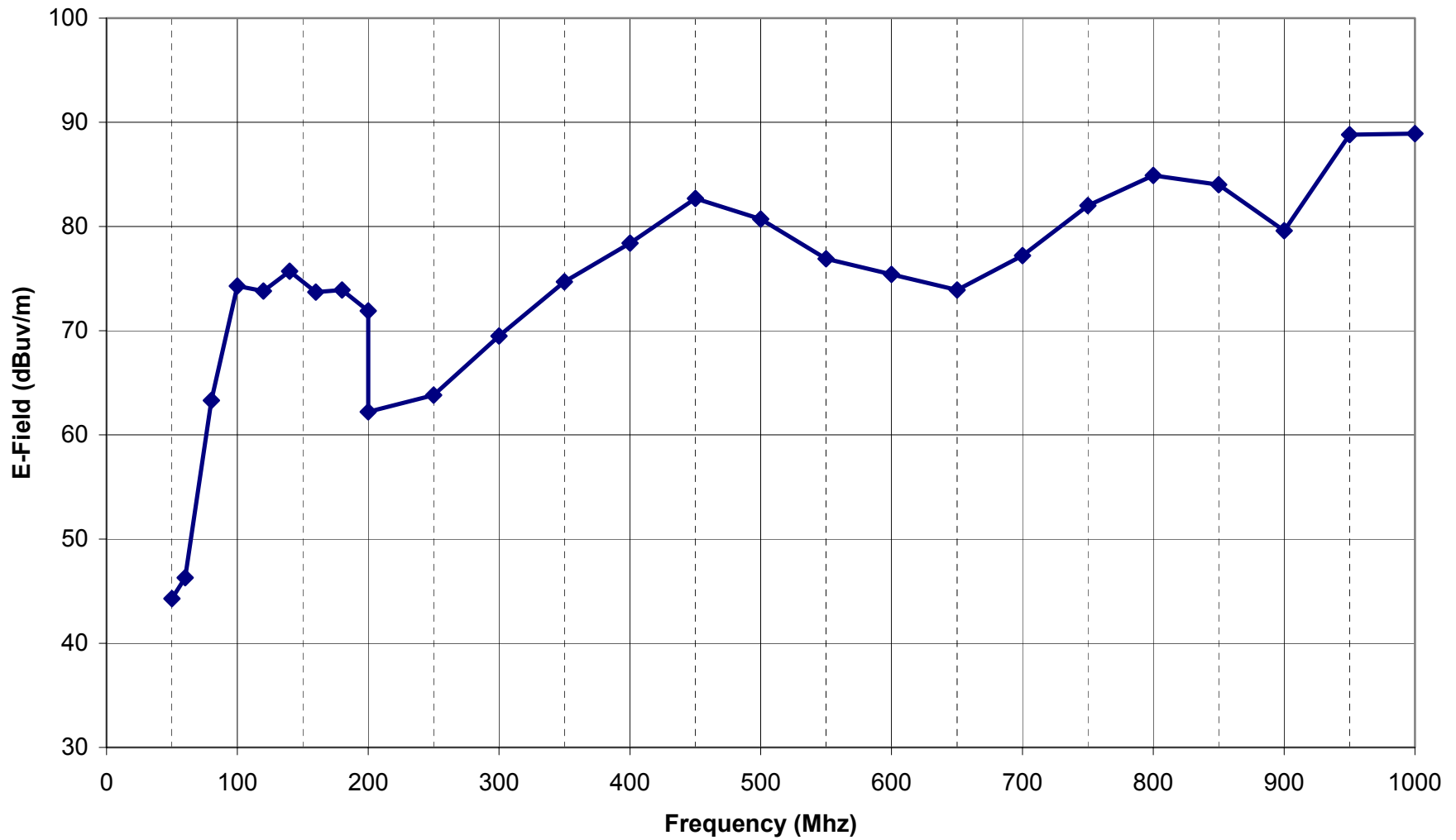
Typical PSDS Radiated E-Field at 1.5 m Horizontal Polarization (Gap Voltage = 1.0v) Receive Antenna 1m Above Ground -- Sphere 0.8m Above Ground
