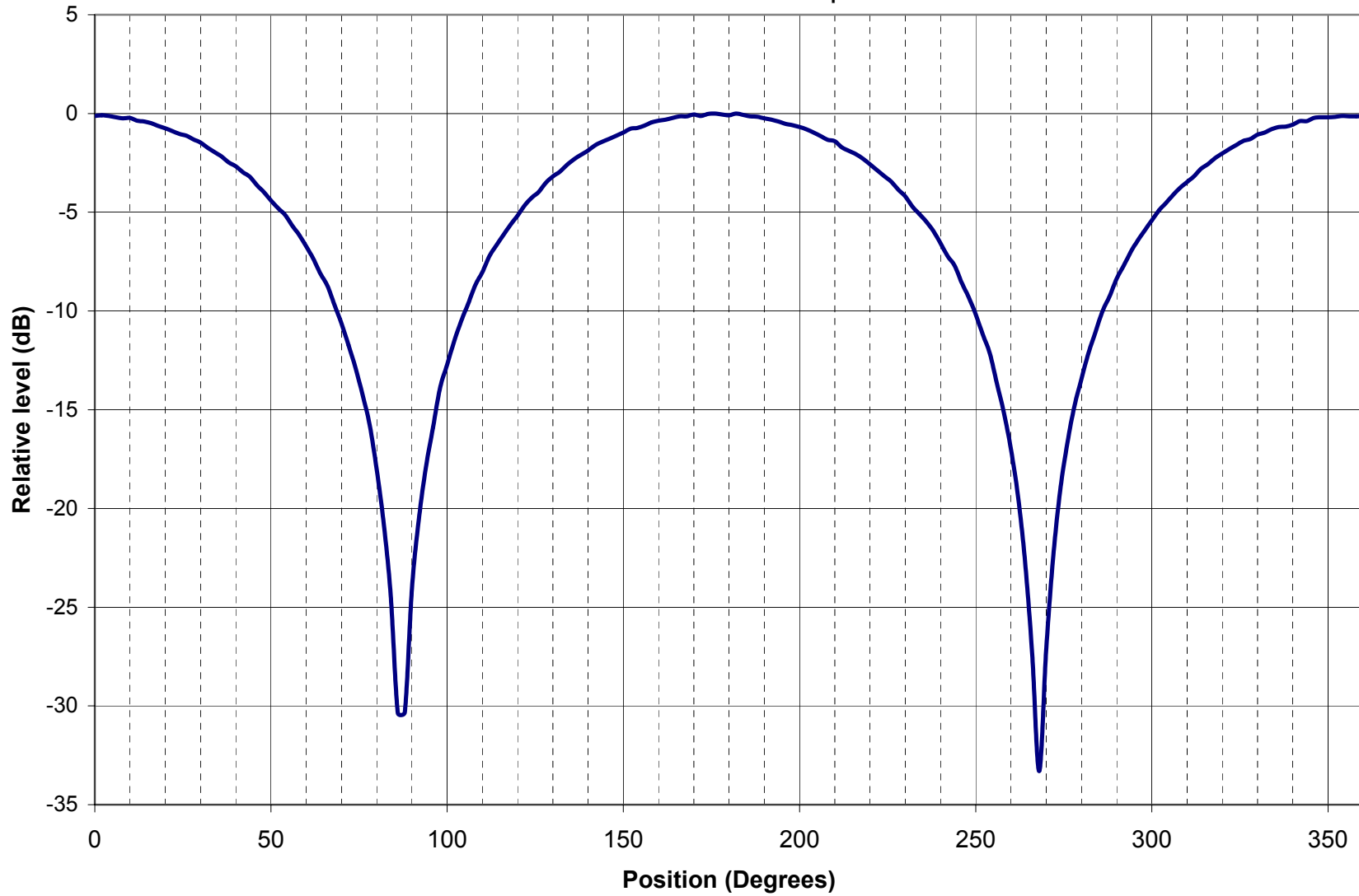
PSDS Radiation Pattern (Horizontal) 500 MHz Tail-Up
